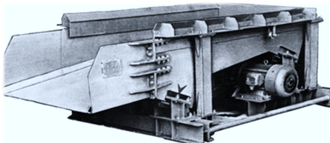
Figure 1 – Vibratory feeder of the VPR-4m type with the rubber elastic suspension (BRM type)
