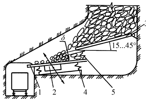
1 – drive section; 2 – vibration exciter; 3 – platform; 4 – elastic supports of the drive section; 5 – elastic drive element C_1 ; \delta – gap
